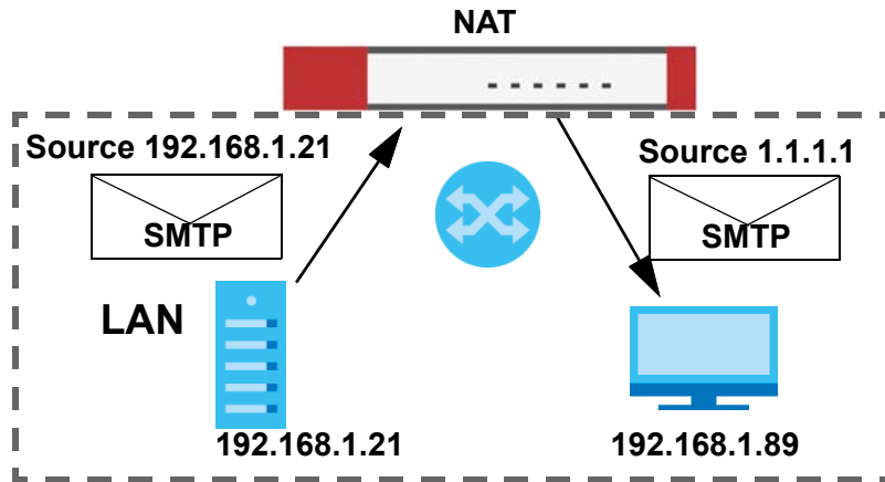
Figure 327 LAN to LAN Return Traffic
