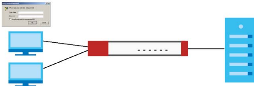
Figure 638 RADIUS Server Network Example
