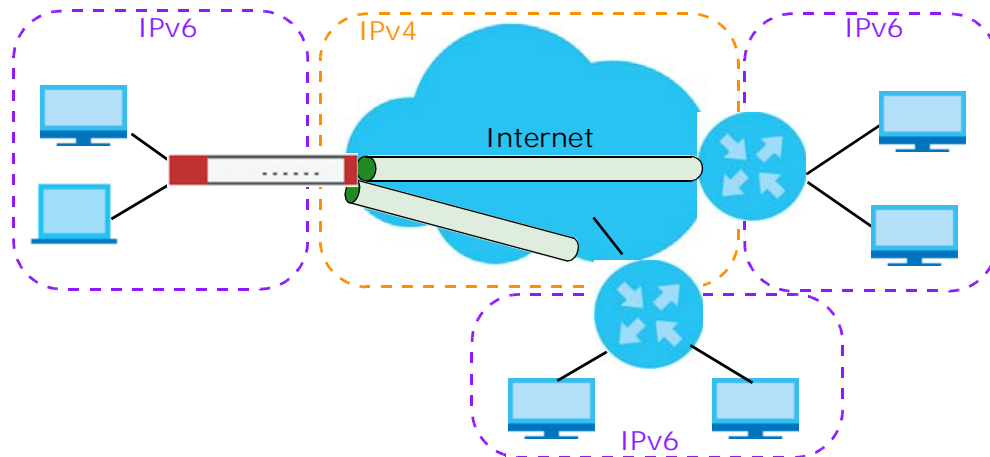
Figure 279 6to4 Tunnel
