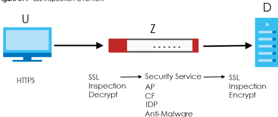
Figure 571 SSL Inspection Overview
