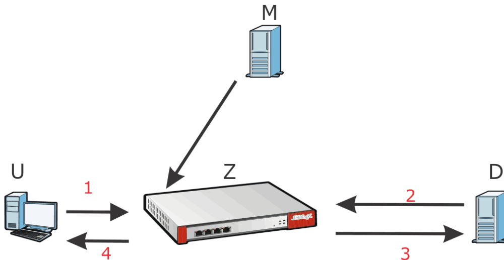
Figure 576 SSL Inspection Certificate Update Overview
