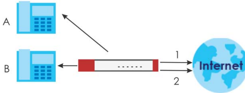
Figure 340 VoIP with Multiple WAN IP Addresses
