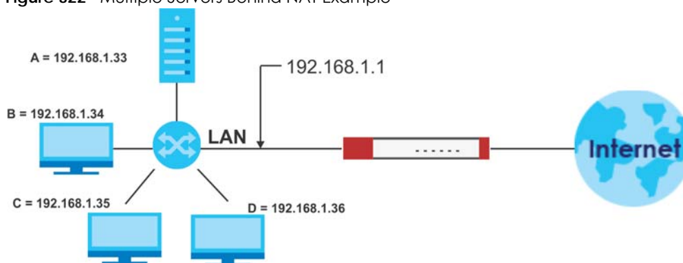
Figure 322 Multiple Servers Behind NAT Example
