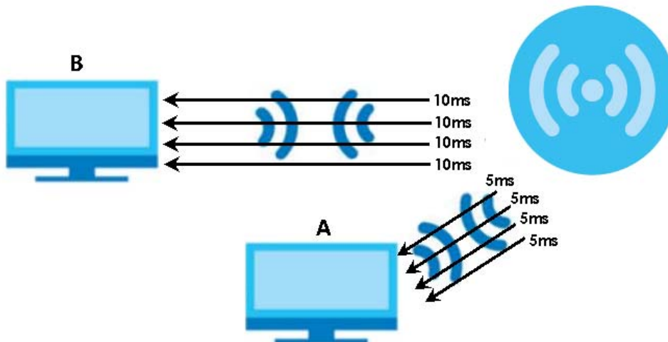
Figure 235 Airtime Fairness Example-Disabled
