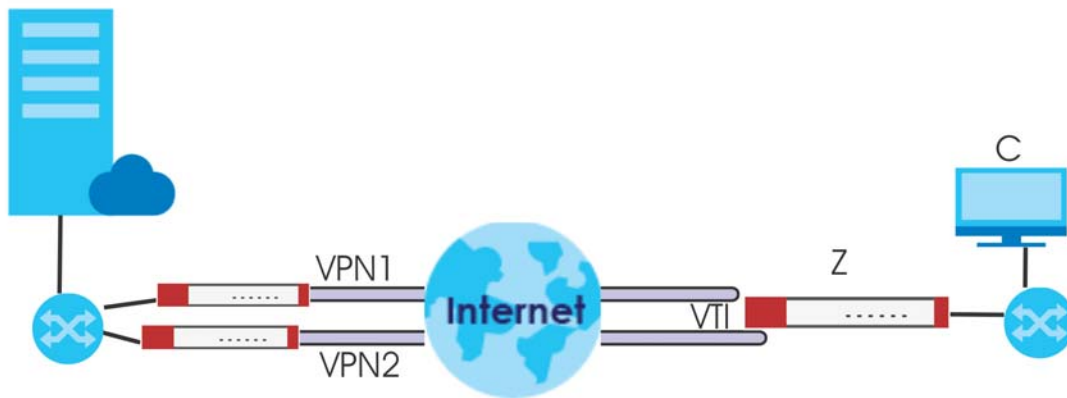
Figure 290 VTI and Trunk for VPN Load Balancing
