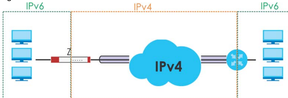
Figure 278 IPv6-in-IPv4 Tunnel
