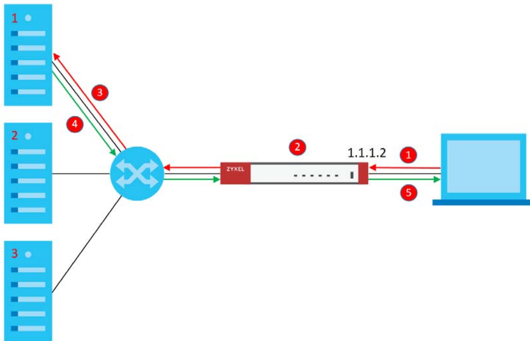
Figure 330 Load Balancing Process
