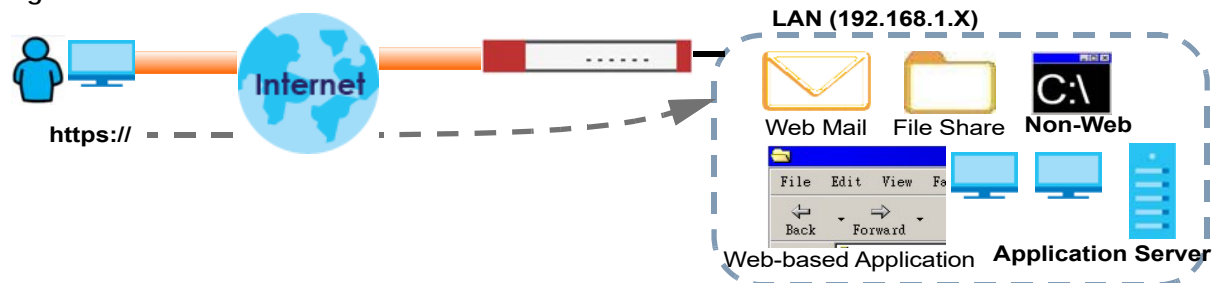
Figure 375 SSL VPN
