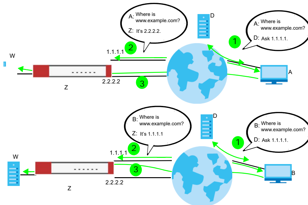
Figure 370 DNS Load Balancing Example
