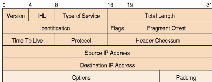
Figure 539 IP v4 Packet Headers
