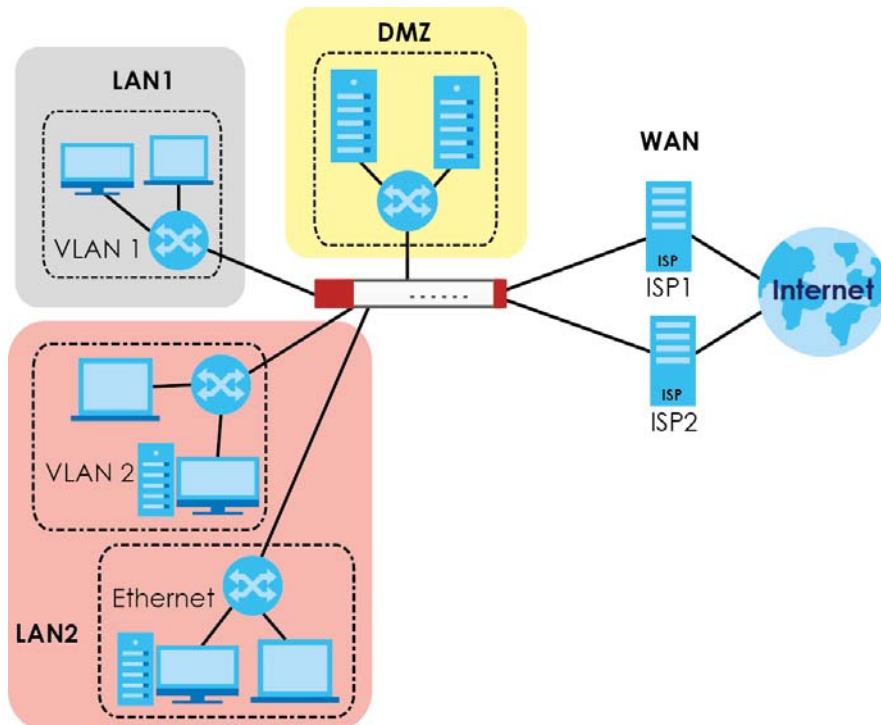
Figure 585 Example: Zones
